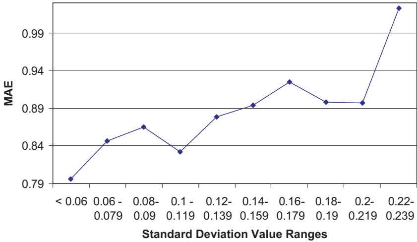
Fig. 8. std-dev MAE analysis.
