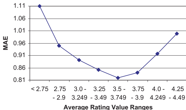
Fig. 7. avg-rating MAE analysis.
