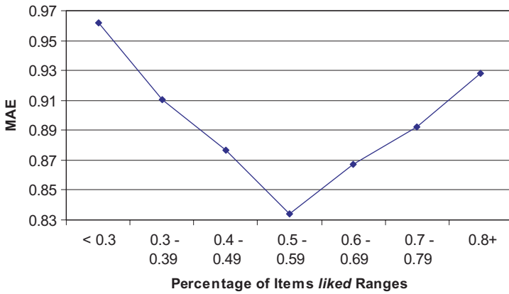
Fig. 5. liked MAE analysis.
