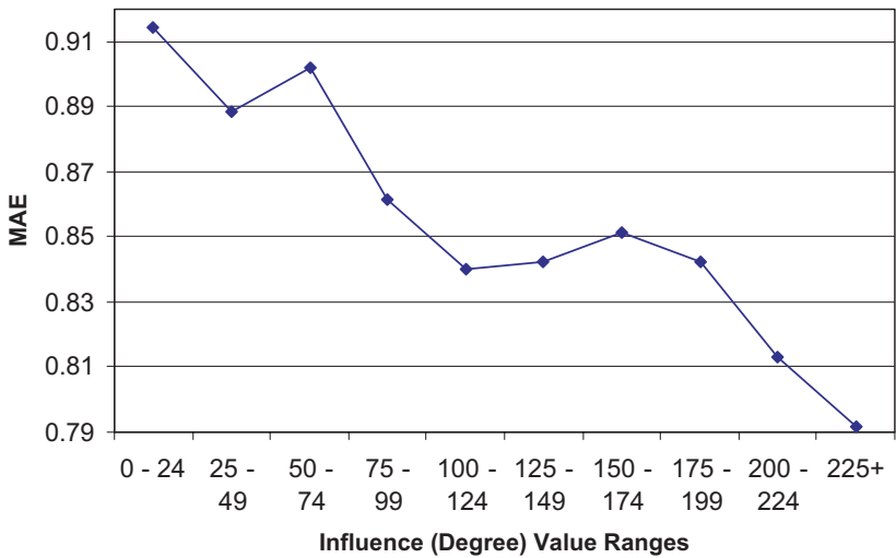
Fig. 9. influence MAE analysis.
