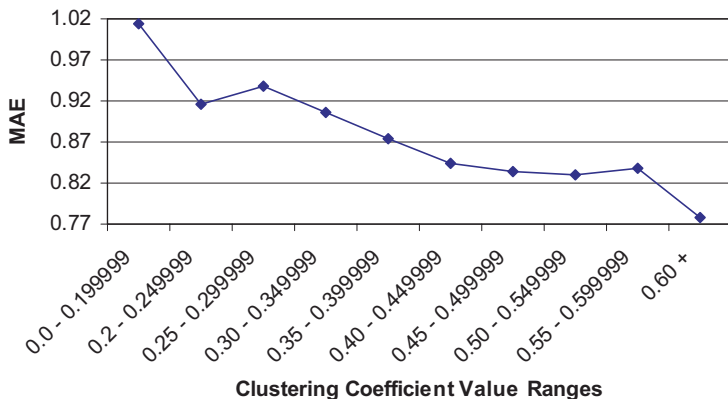
Fig. 10. clustering-coeff MAE analysis.
