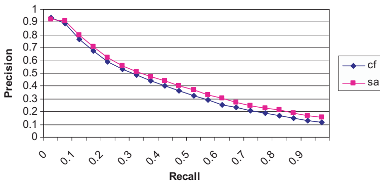
Fig. 11. Comparing spreading activation (sa) and traditional memory-based approaches (cf) to collaborative filtering.
